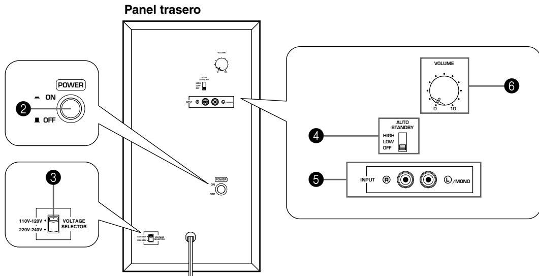
Panel trasero
